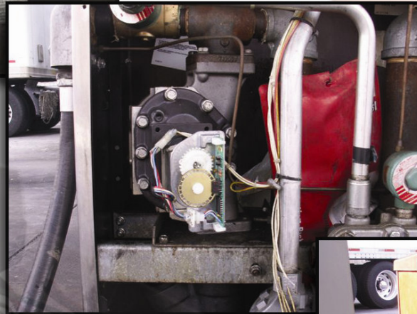
Damaged Pulsars
